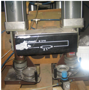
Seam Sealing Mashine with cutter Pfaff made in Geramny
